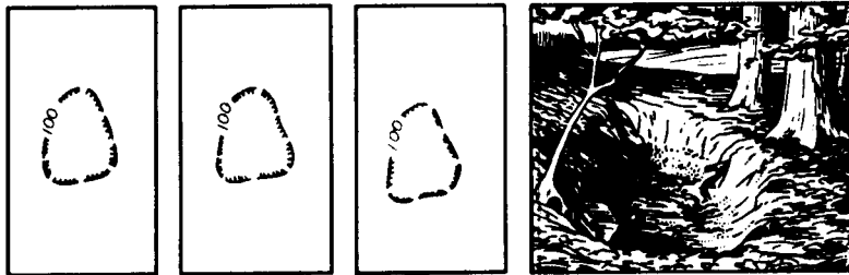
Figure 47. Depression, With Depth Greater Than Contour Interval. The tick marks always point downgrade.
